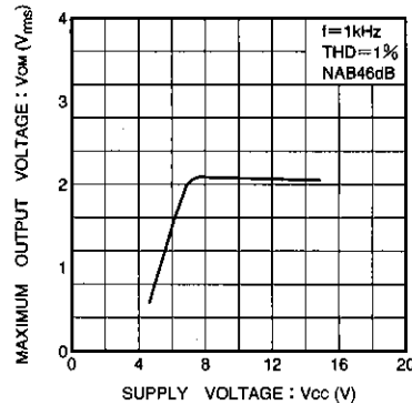
Fig. 8 Maximum output voltage vs. supply voltage
