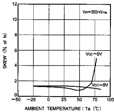
Fig. 6 Detection bandwidth skew vs. ambient temperature characteristic
