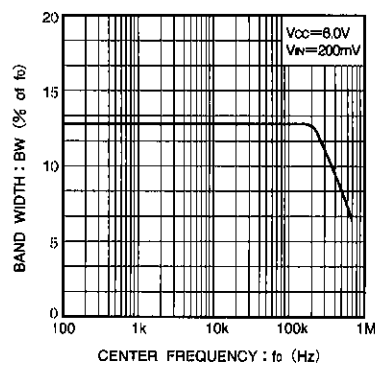
Fig. 4 Detection bandwidth vs. frequency characteristic
