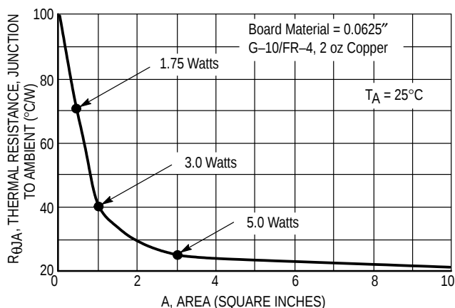
Figure 15. Thermal Resistance versus Drain Pad Area for the D 3 PAK Package (Typical)
