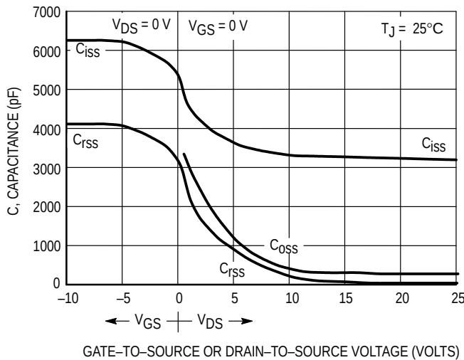
Figure 7a. Low Voltage Capacitance Variation
