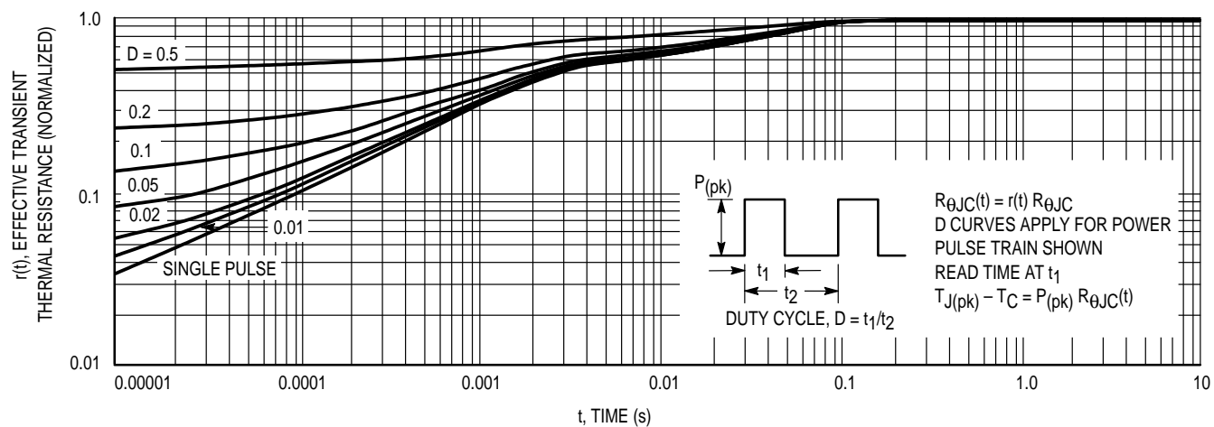
Figure 14. Thermal Response
