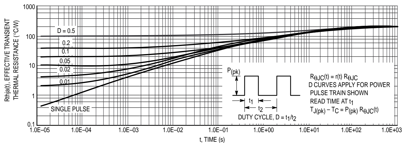
Figure 15. Thermal Response
