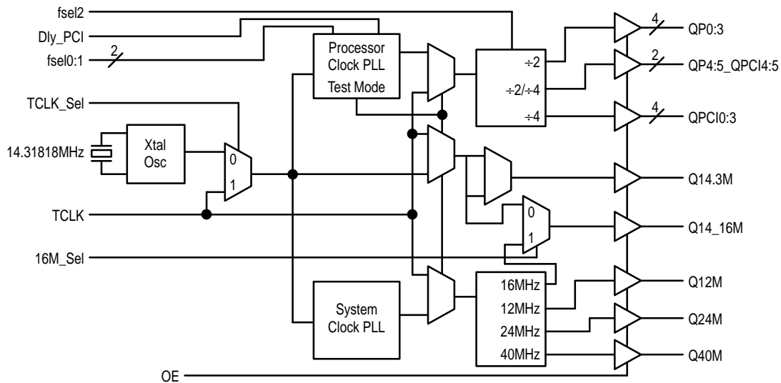
Figure 1. Logic Diagram
