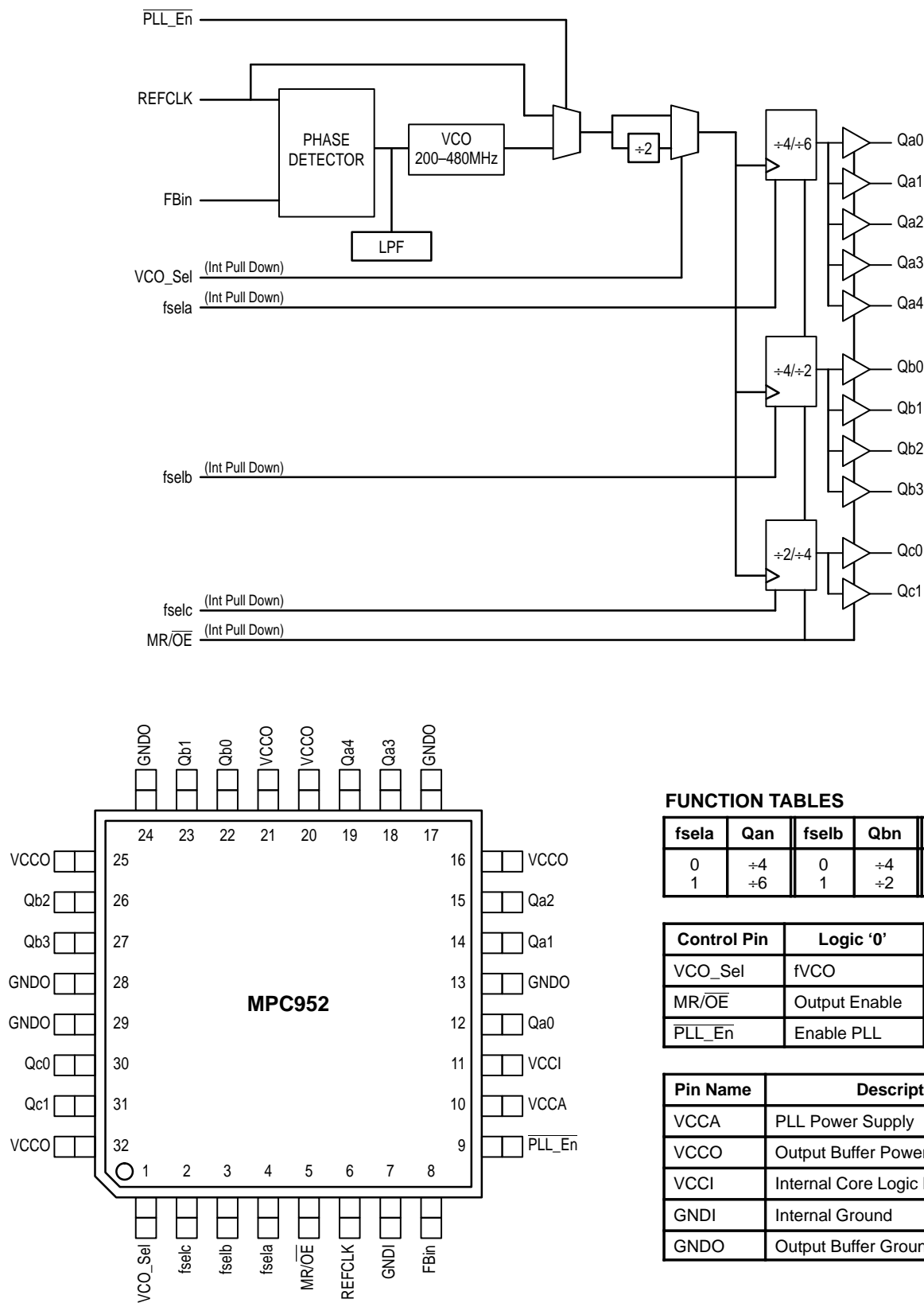
Figure 2. 32-Lead Pinout (Top View)
