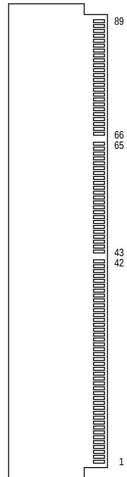
178-LEAD CARD EDGE TOP VIEW CASE TBD
