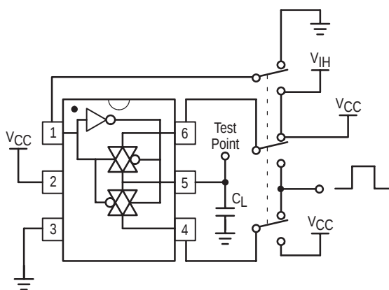
Figure 5. Propagation Delay Test Set-Up, Analog I/O to Analog I/O
