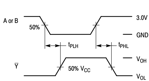
Figure 4. Switching Waveforms
