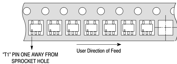
Figure 15. DTT1 and DTT3 (TSOP5) Reel Configuration/Orientation
