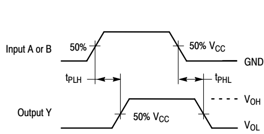
Figure 4. Switching Waveforms
