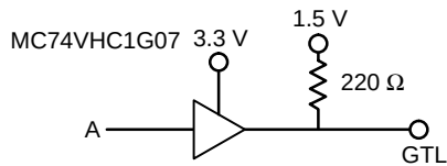
Figure 9. GTL Driver
