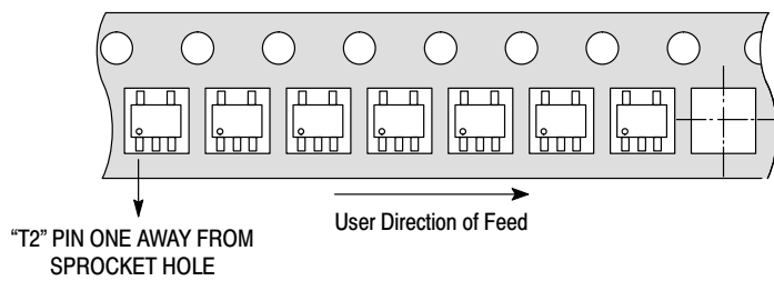
Figure 14. DFT2 and DFT4 (SC88A) Reel Configuration/Orientation
