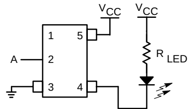
Figure 8. LED Driver
