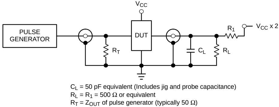
Figure 6. Test Circuit
