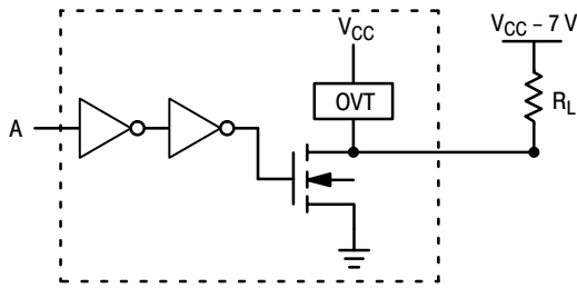
Figure 4. Output Voltage Mismatch Application
