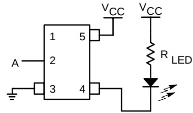
Figure 8. LED Driver
