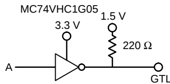
Figure 9. GTL Driver
