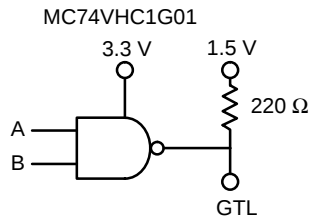
Figure 9. GTL Driver
