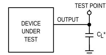
Figure 2. Test Circuit
