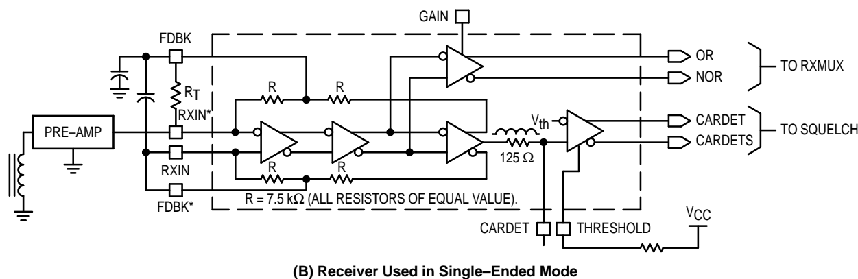
Figure 4-1. Receiver Amplifier With Carrier Detect
