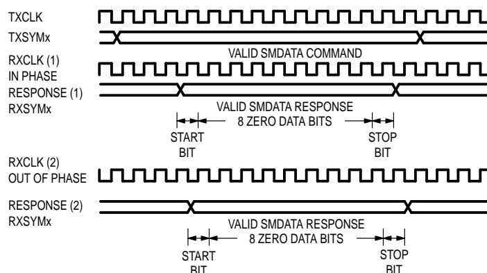
Figure 8–2. SMDATA Command Response Time
