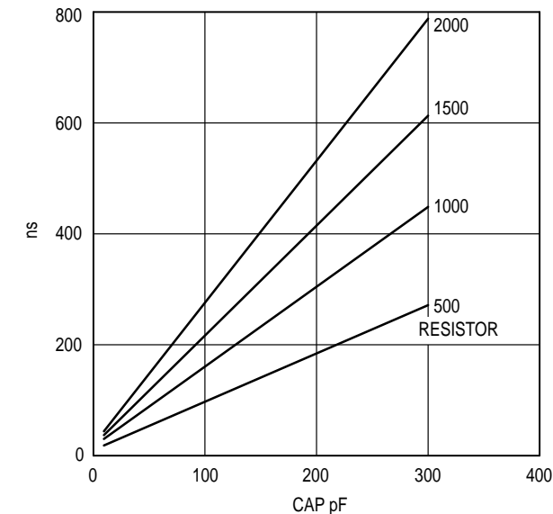
Figure 9-3. One Shot Pulse Width versus Rext/Cext
