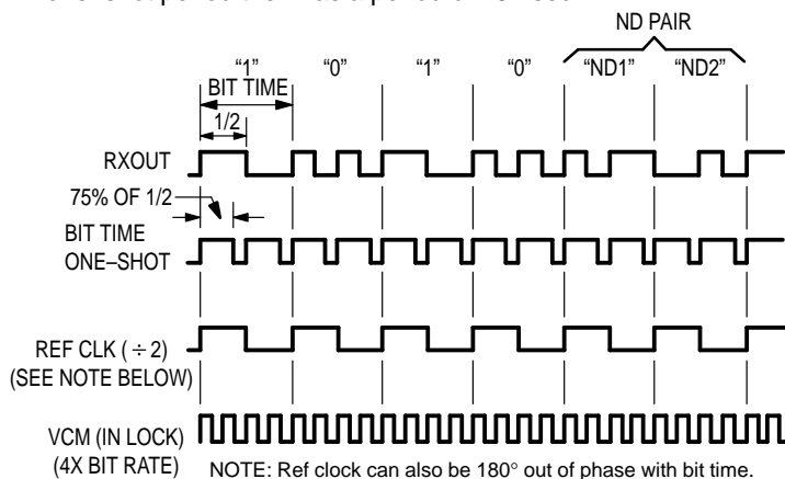
Figure 5–2. Clock Recovery Timing Signals
