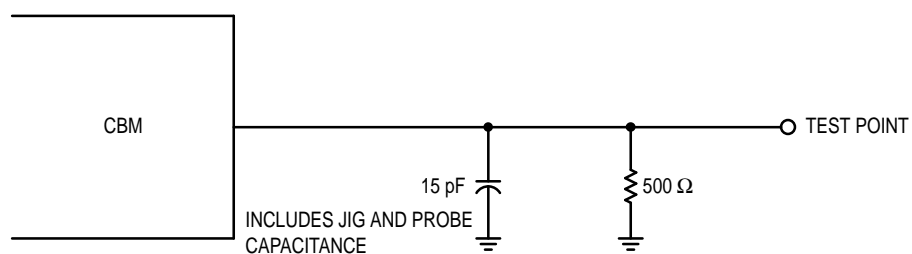
Figure 9-2. TTL, TXOUT, TXOUT*, Up* &amp; Down* AC Test Load
