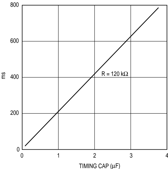
Figure 9-7. Jabber Time Constant versus Capacitance
