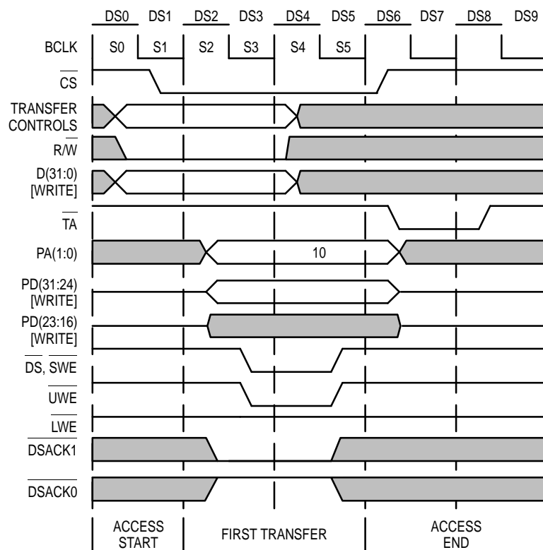
Figure 46. 8-Bit '040 WRITE to 16-Bit Peripheral Example (PA1,PA0=10)
