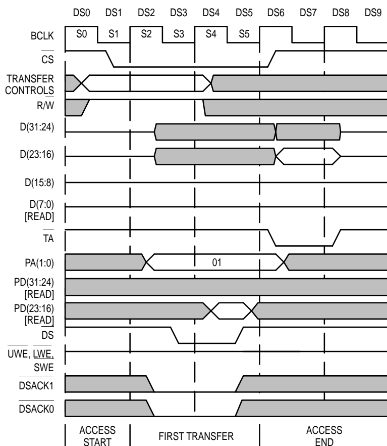
Figure 51. 8-Bit '040 READ From 32-Bit Peripheral Example (PA1,PA0=01)
