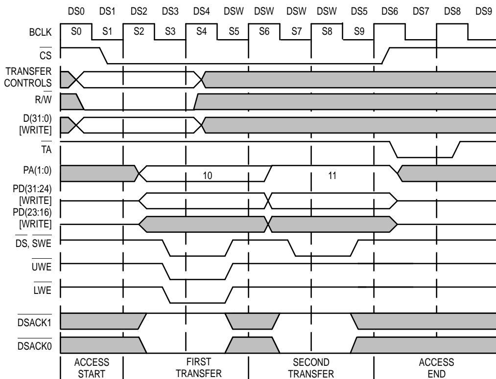
Figure 24. 16-Bit '040 WRITE to 8-Bit Peripheral Example (PA1=1)
