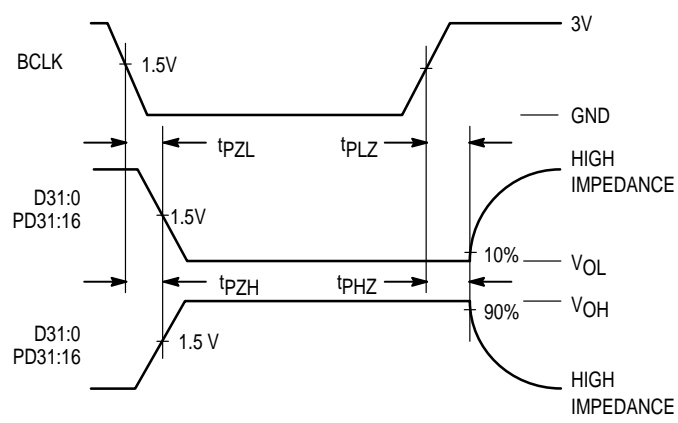
Figure 10. Enable/Disable Times
