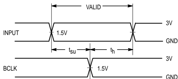
Figure 11. Setup/Hold Times
