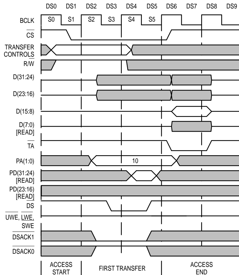
Figure 45. 8-Bit '040 READ From 16-Bit Peripheral Example (PA1,PA0=10)
