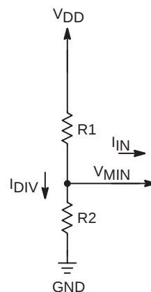
Figure 5. V_{MIN} Circuit
