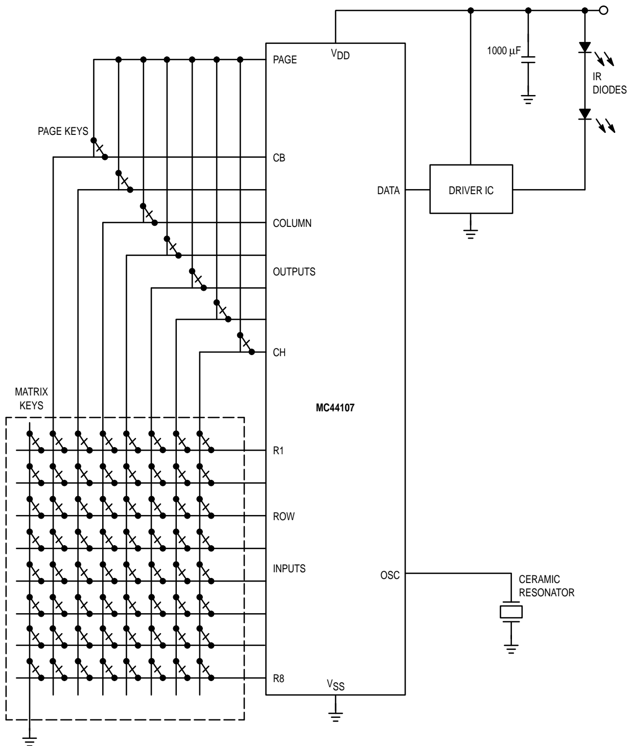
Figure 3. Transmitter Circuit
