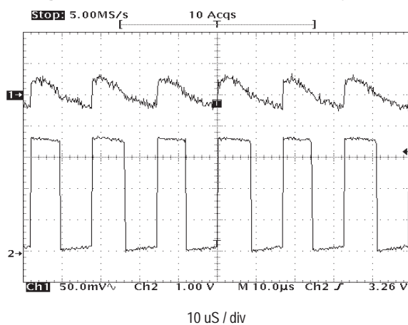
Figure 15. VMAIN Output Ripple (Heavy Load)
