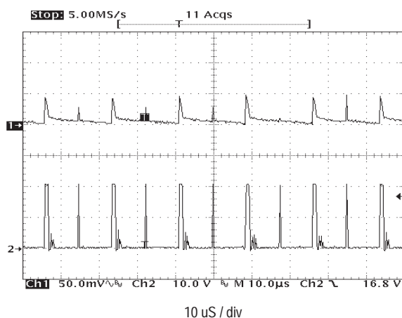
Figure 17. VAUX Output Ripple (Heavy Load)
