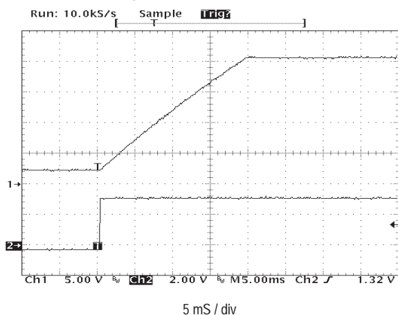
Figure 19. VAUX Startup
