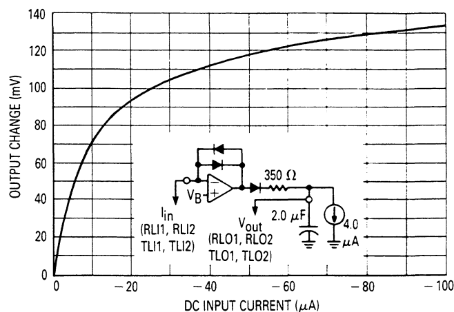
FIGURE 11 — LEVEL DETECTOR DC TRANSFER CHARACTERISTICS
