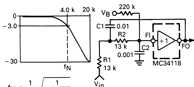
FIGURE 9 — LOW PASS FILTER
