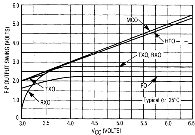
FIGURE 22 — TYPICAL OUTPUT SWING versus V_{CC}
