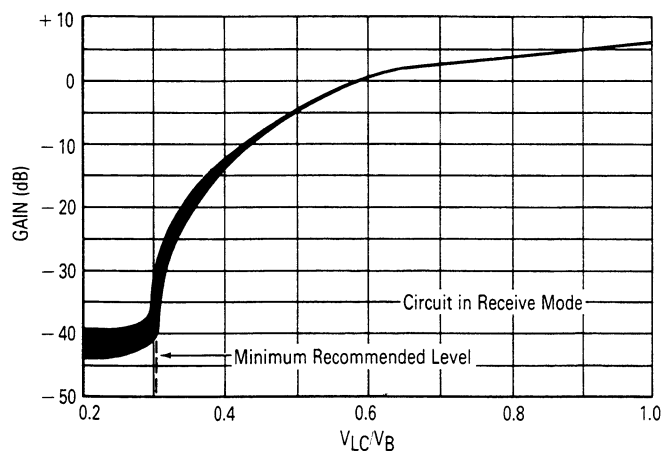
FIGURE 14 — RECEIVE ATTENUATOR versus VOLUME CONTROL
