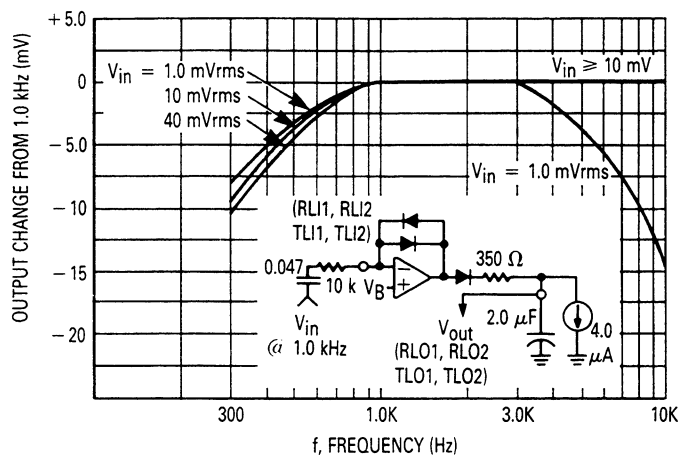
FIGURE 13 — LEVEL DETECTOR AC TRANSFER CHARACTERISTICS versus FREQUENCY
