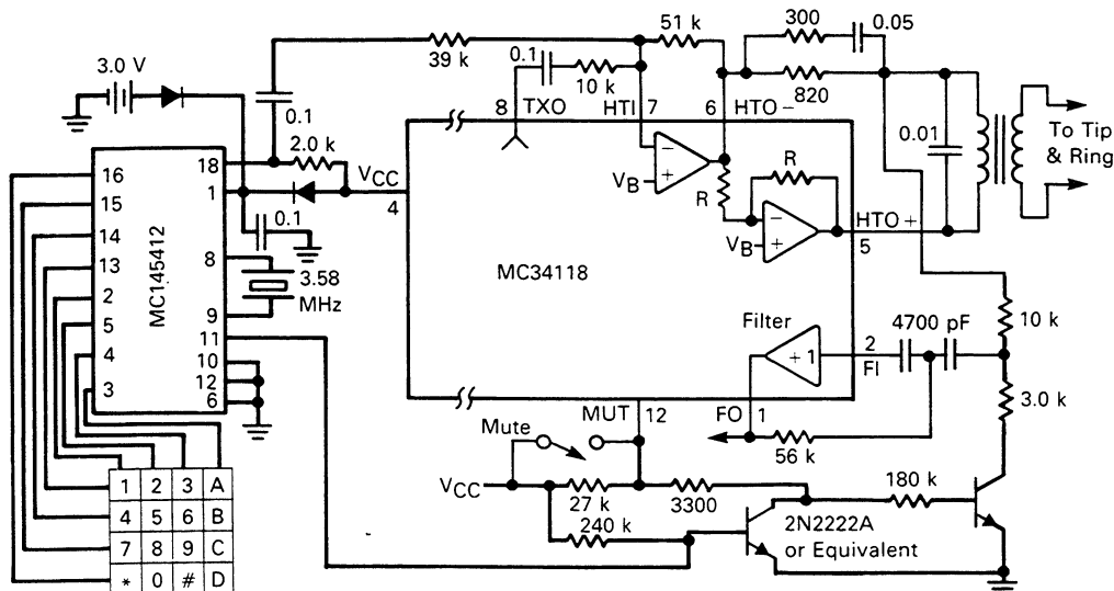
FIGURE 32 — ADDING A DIALER TO THE SPEAKERPHONE
