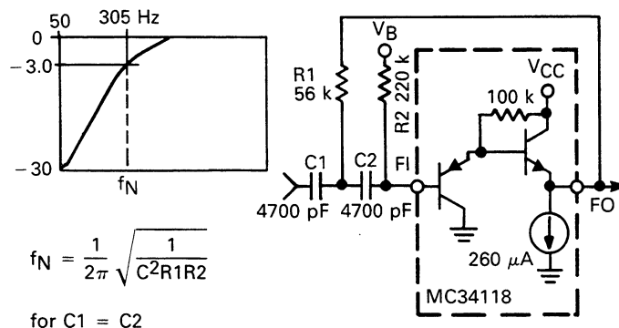
FIGURE 8 — HIGH PASS FILTER
