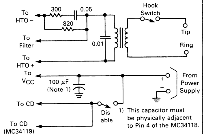
FIGURE 31 — OPERATING FROM A POWER SUPPLY
