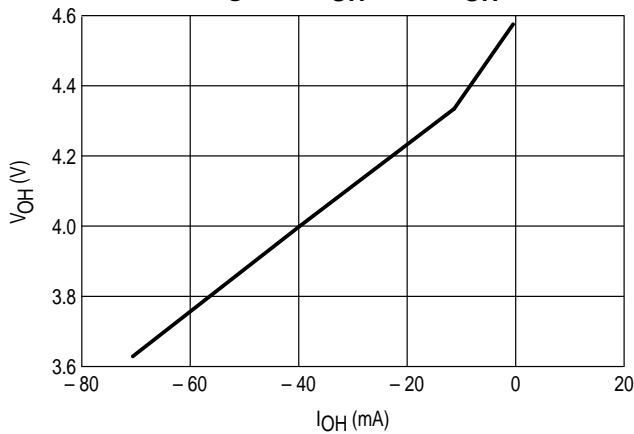
Figure 5. V_{OH} versus I_{OH}
