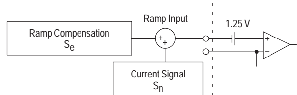
Figure 20. Ramp Compensation
