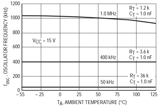
Figure 2. Oscillator Frequency versus Temperature
