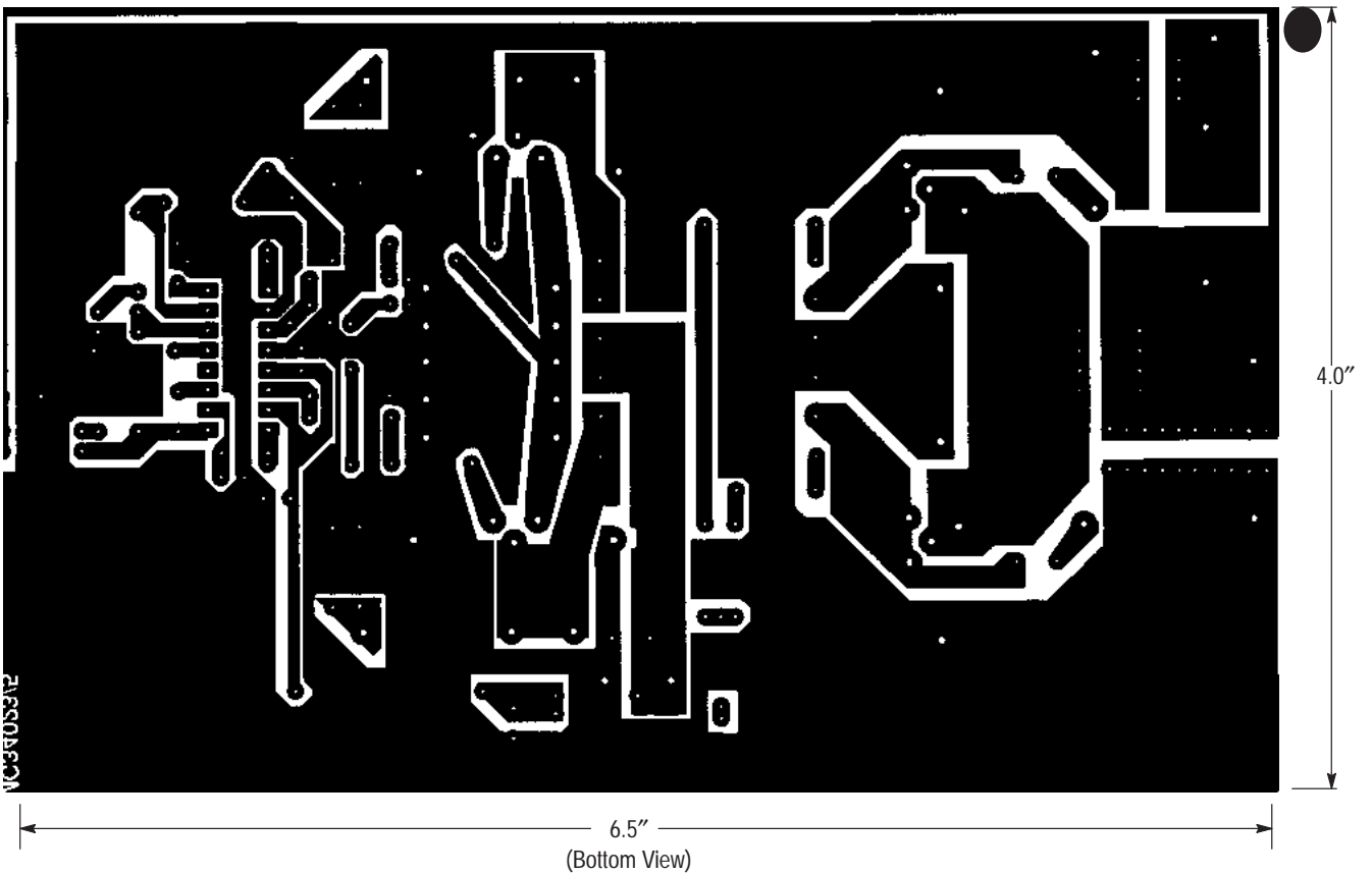
Figure 38. PC Board Without Components
