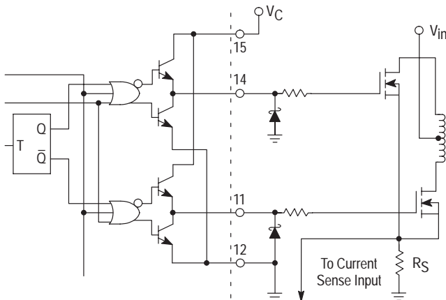
Figure 35. MOSFET Parasitic Oscillations
