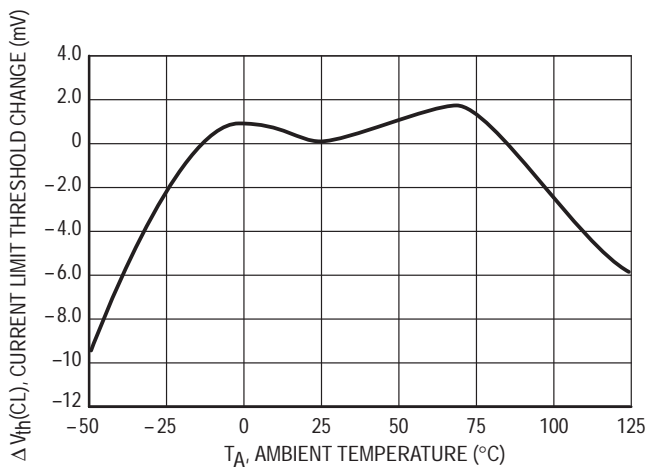
Figure 11. Current Limit Comparator Threshold Change versus Temperature
