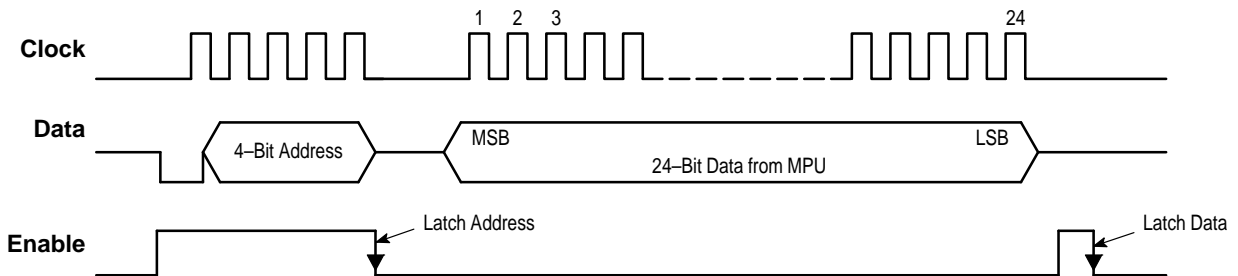
Figure 2. Writing Data to the MC33410
