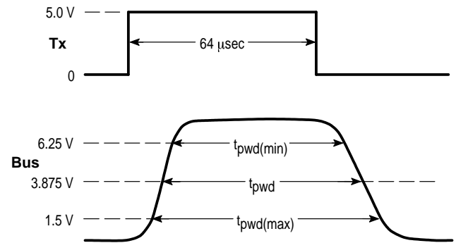
Figure 3. Pulse Width Distortion
