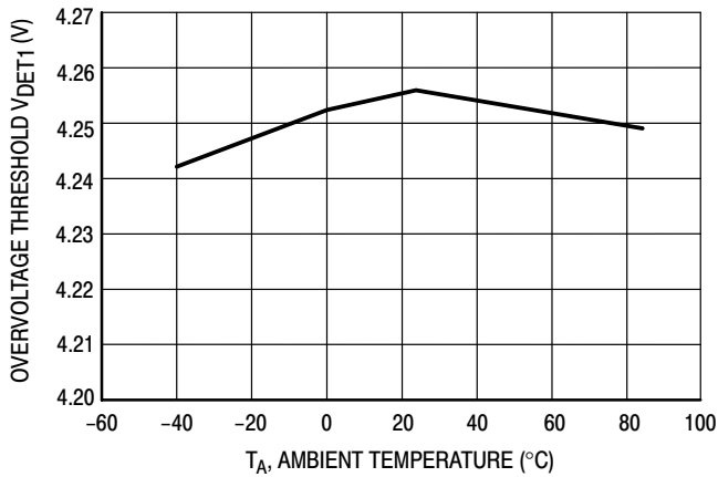
Figure 3. Overvoltage Threshold vs Temperature MC33349N-3X
