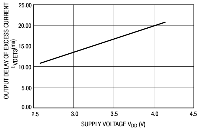
Figure 19. Excess Current Delay Time vs V DD MC33349N-3X
