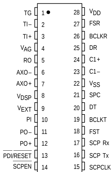
28-LEAD PDIP, SOG
