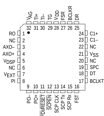
32-LEAD TQFP
