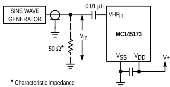
Figure 11. Test Circuit
