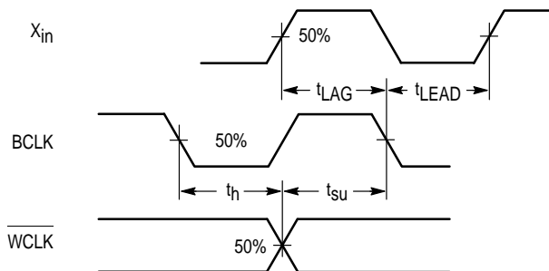
Figure 6. \overline{WCLK} Timing ( DMODE = 1 , WDLY = 1 )
