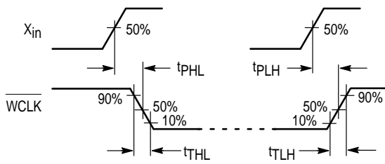
Figure 3. \overline{WCLK} Out Propagation Delay Timing (Master Mode)
