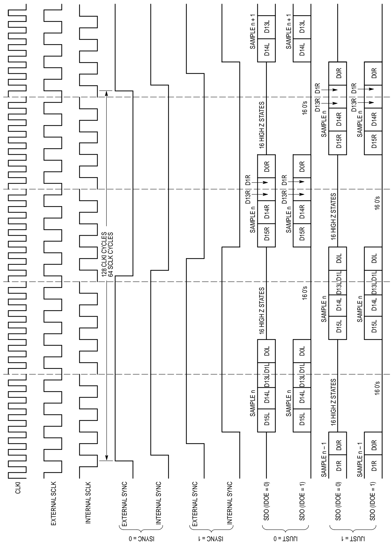
Figure 11. Serial Interface Operation with MC145073 Configured as Slave (ISLAV = 1)
