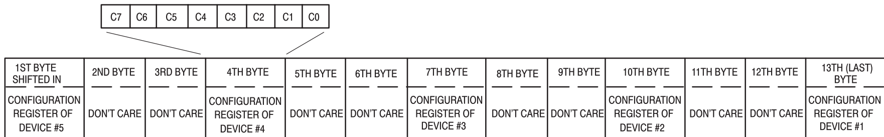
(b) Configuration Registers
