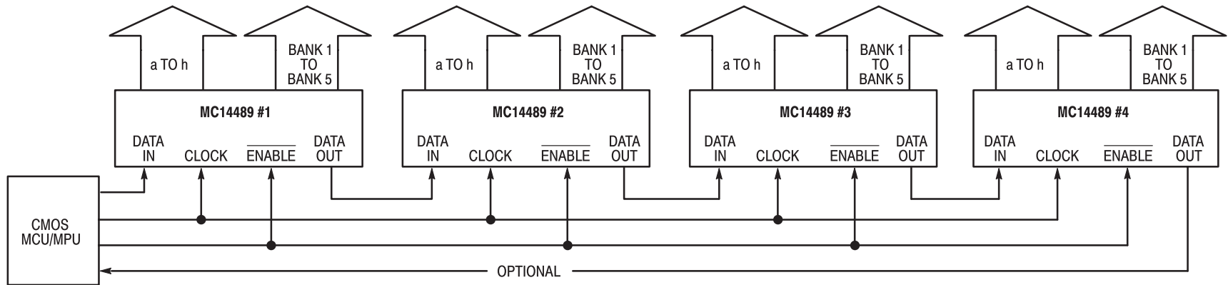
(a) Cascading Four Devices
