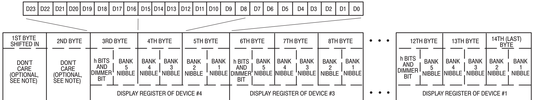
(c) Display Registers
