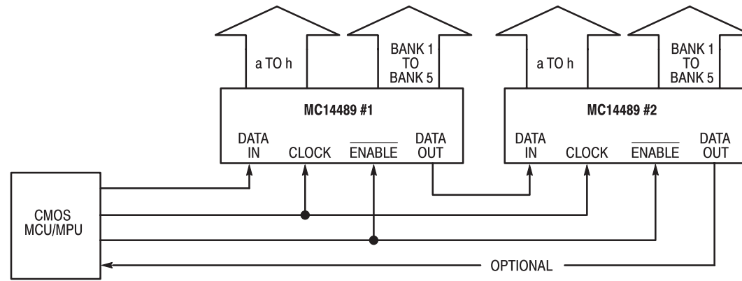
(a) Cascading Two Devices
