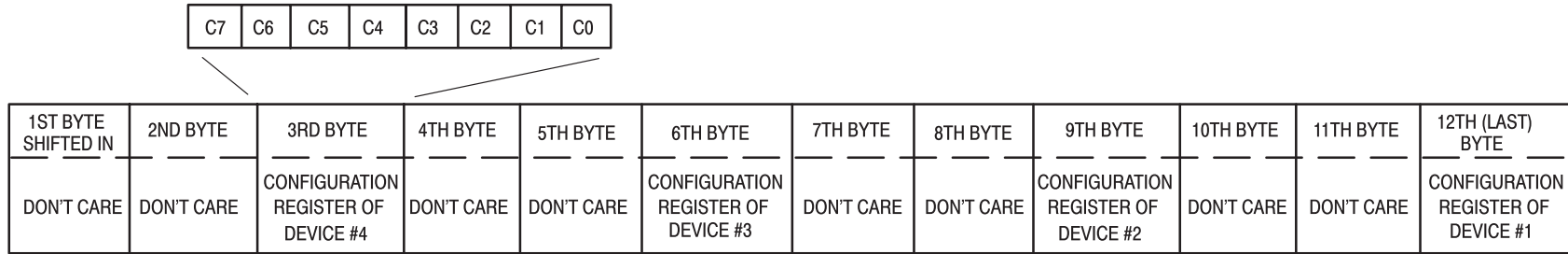
(b) Configuration Registers
