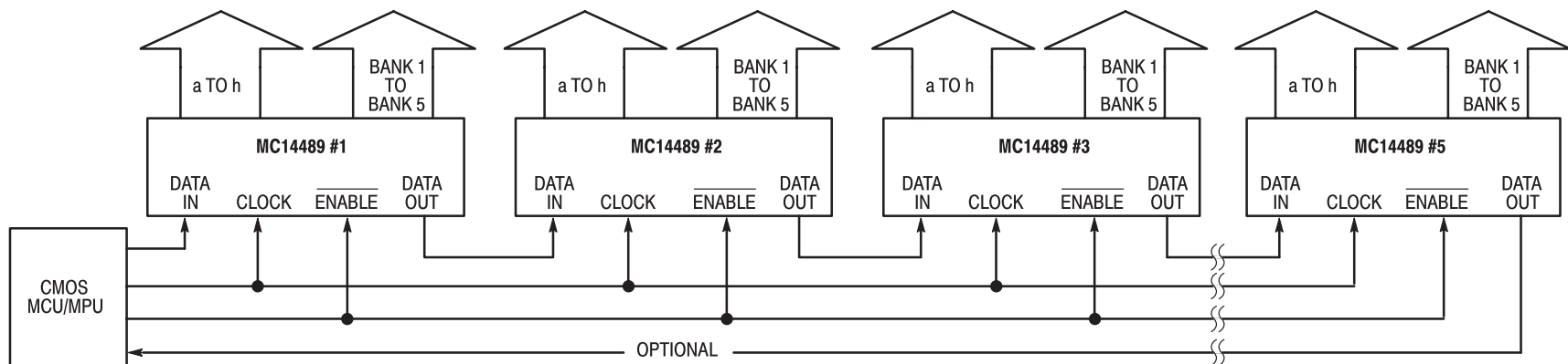
(a) Cascading Five Devices
