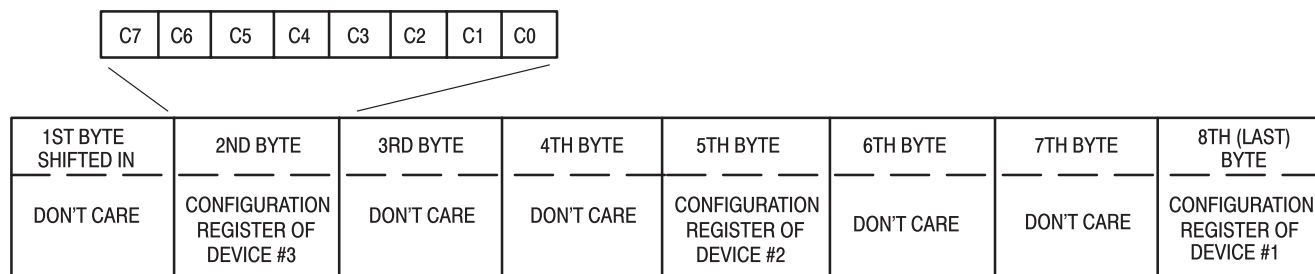
(b) Configuration Registers
