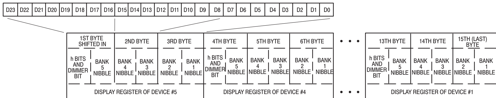
(c) Display Registers
