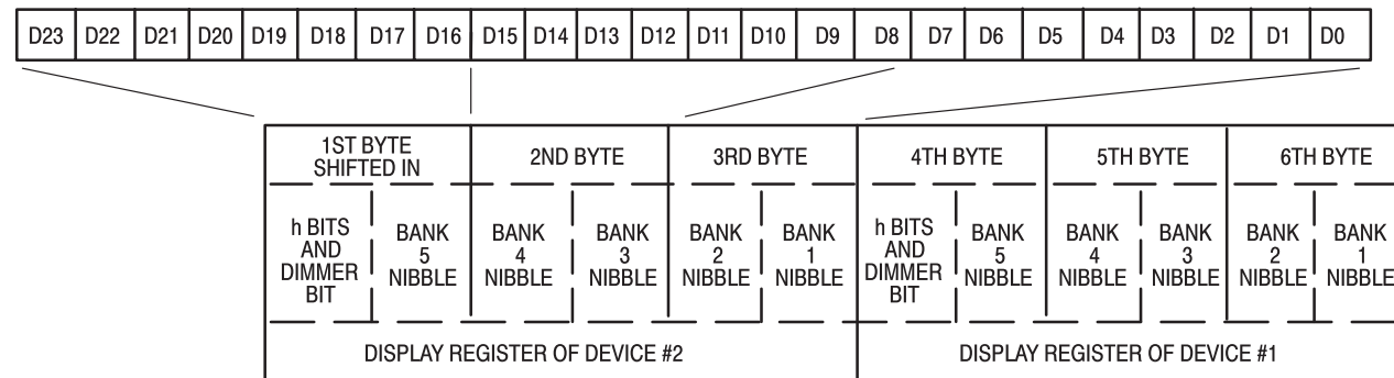
(c) Display Registers
