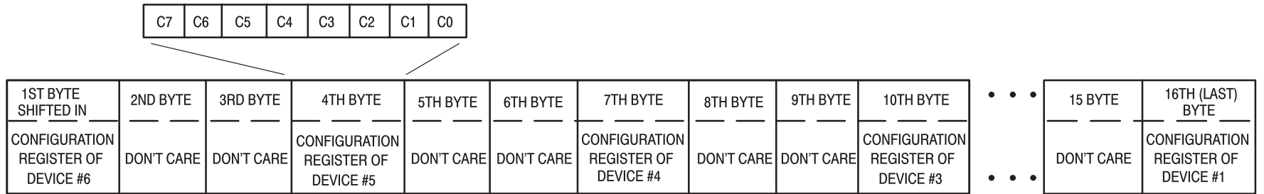
Figure 14. Bit Stream Formats for Six Devices Cascaded
