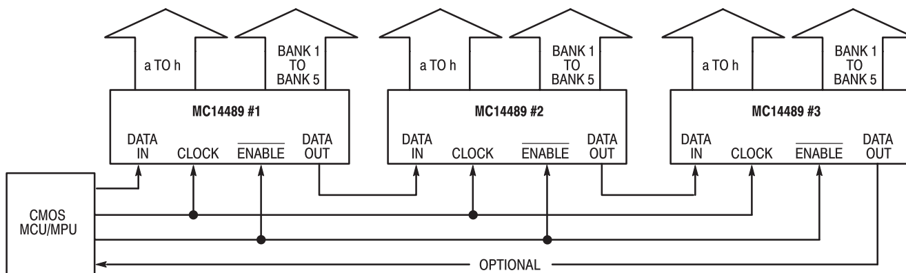
(a) Cascading Three Devices
