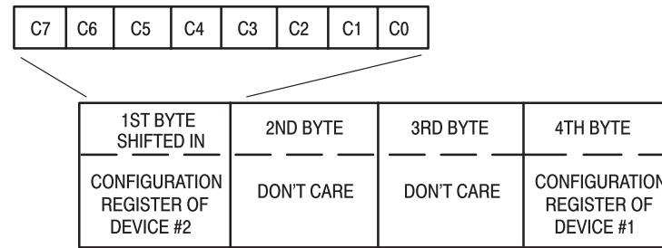
(b) Configuration Registers
