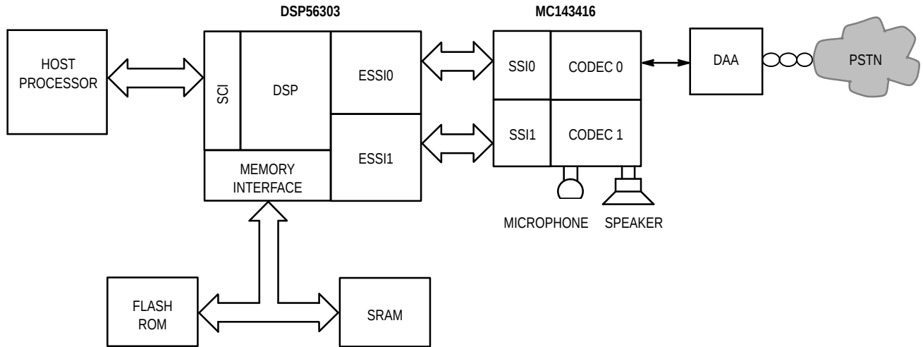
Figure 10. Active DSP-Based Modem Application
