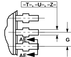
DETAIL AA
