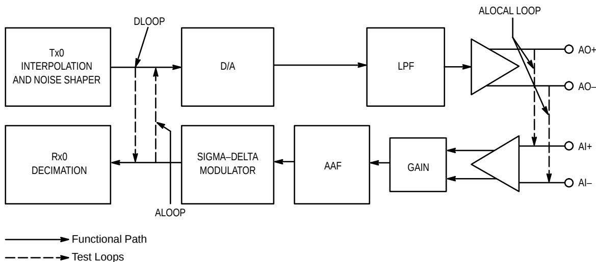
Figure 2. Digital and Analog Loopback Features
