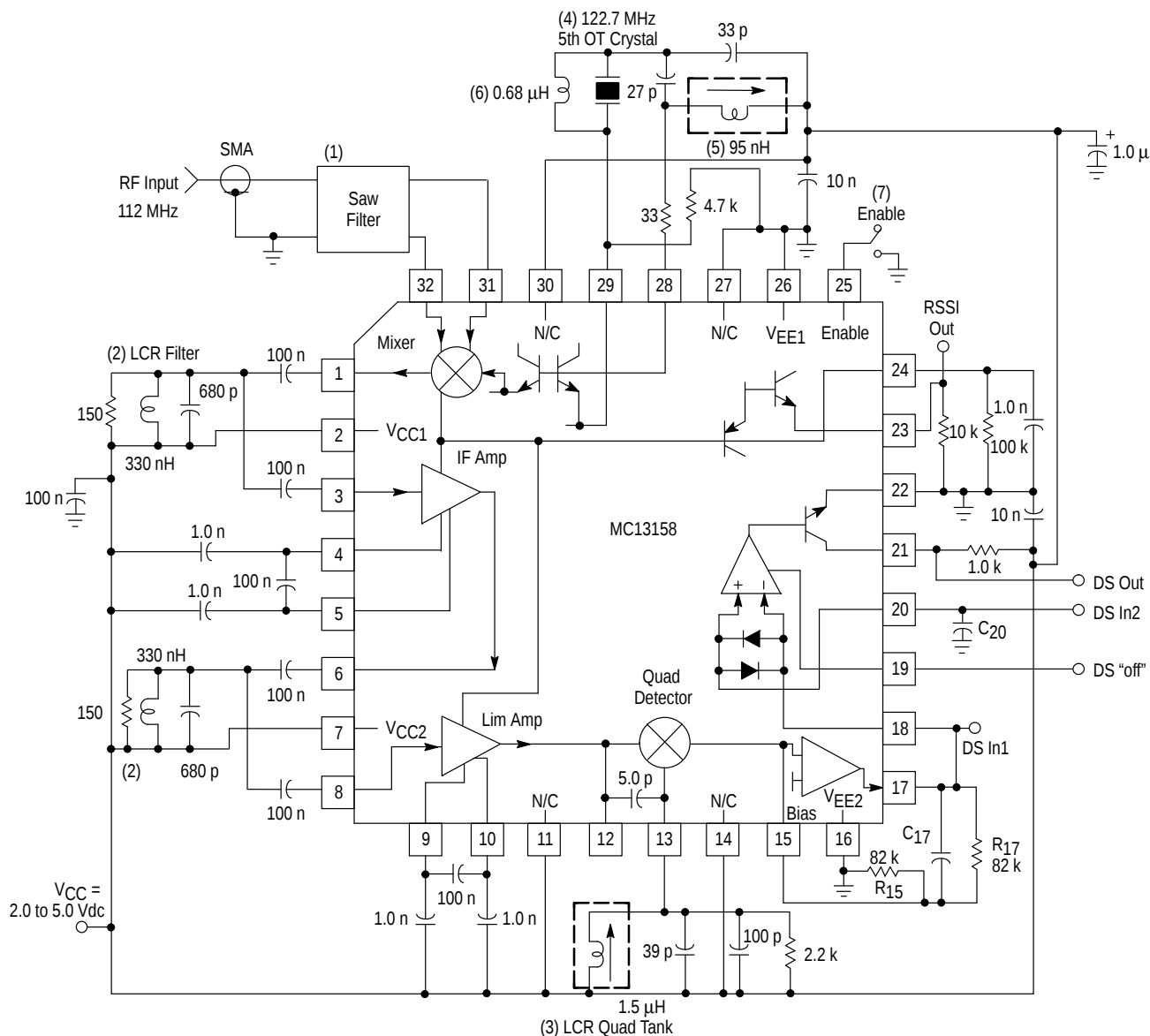
Figure 12. Application Circuit
