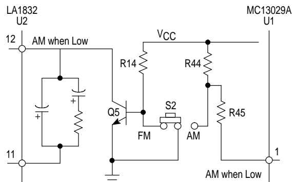
Figure 20. AM/FM Switch
