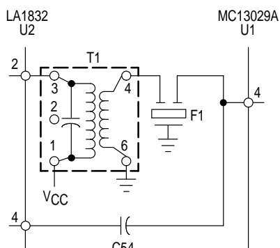
Figure 21. IF Connection
