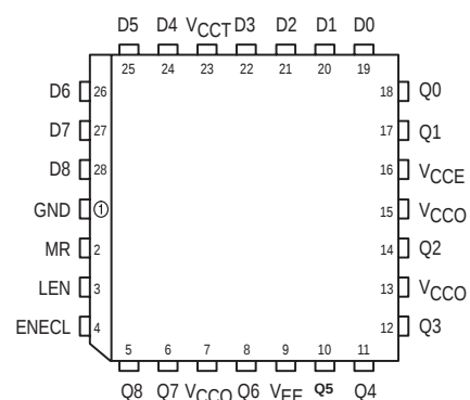
Pinout: 28-Lead PLCC (Top View)
