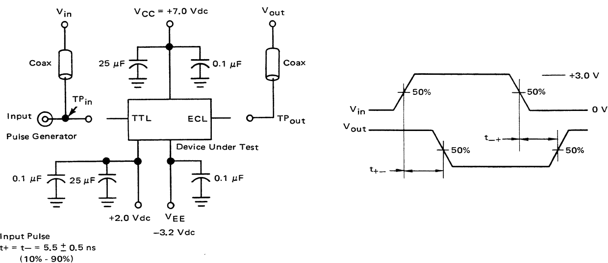
FIGURE 2 — SWITCHING TIME TEST CIRCUIT AND WAVEFORMS @ 25°C FOR PROPAGATION DELAY FROM TTL INPUT TO ECL OUTPUT
