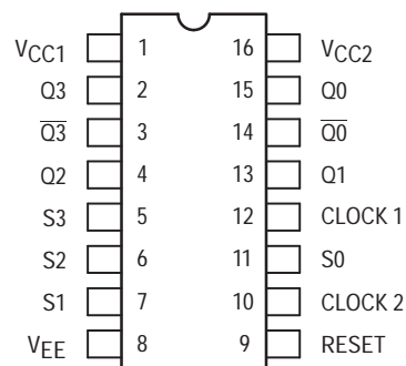
DIP PIN ASSIGNMENT
