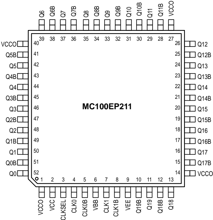
Pinout: 52-Lead TQFP (Top View)
