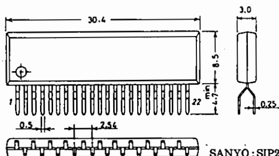
Package Dimensions 3066 (unit: mm)
