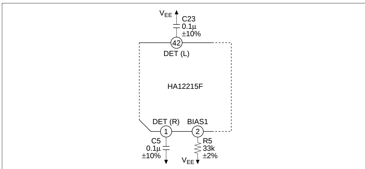
Figure 7 Tolerance of External Components
