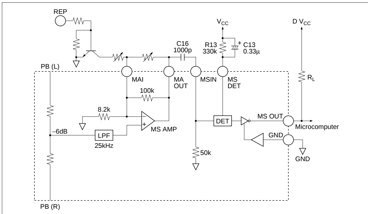
Figure 4 Music Sensor Block Diagram
