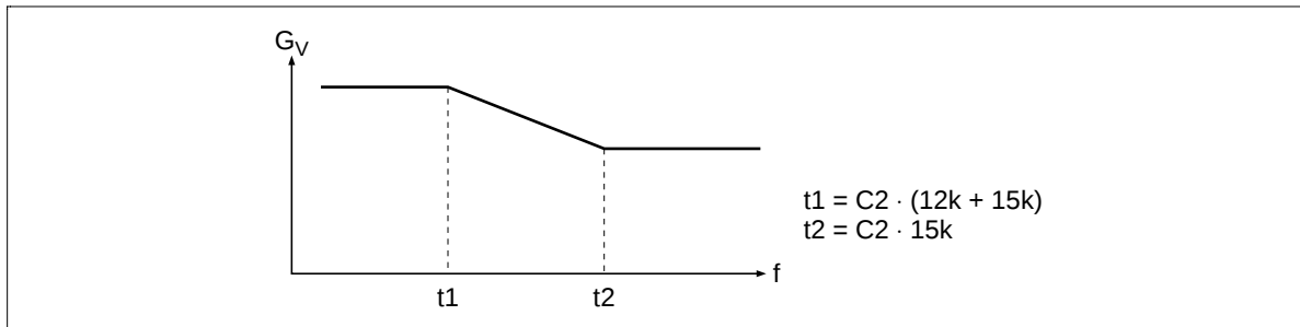
Figure 3 Frequency Characteristic of PB Equalizer
