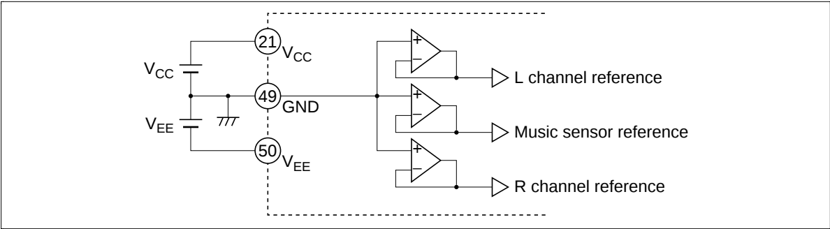
Figure 1 Reference Voltage
