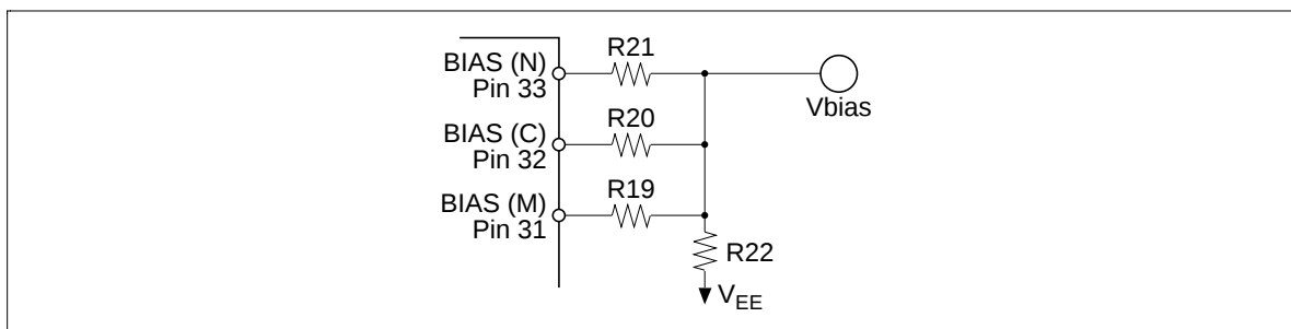
Figure 10 External Components of Bias Block
