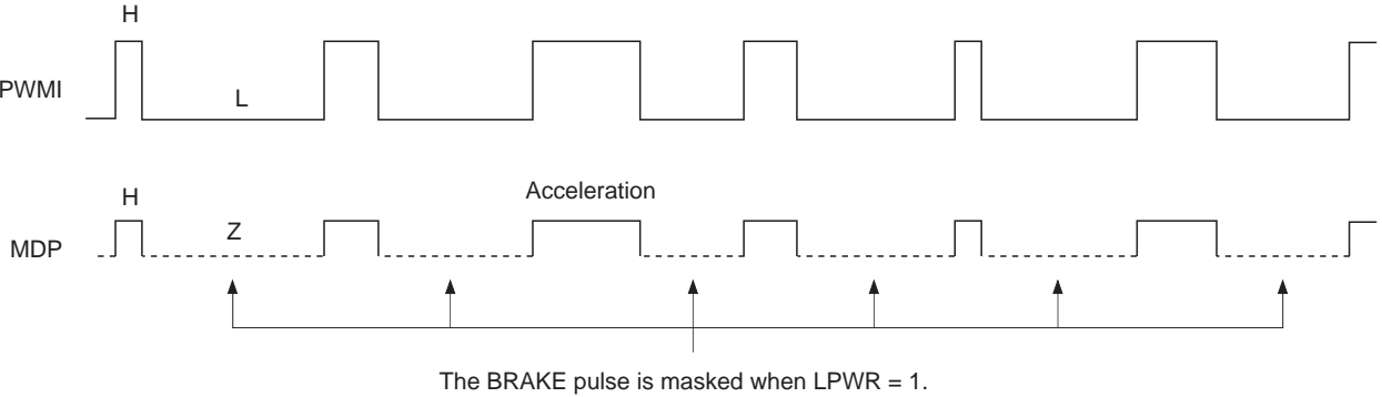
Timing Chart 1-20
