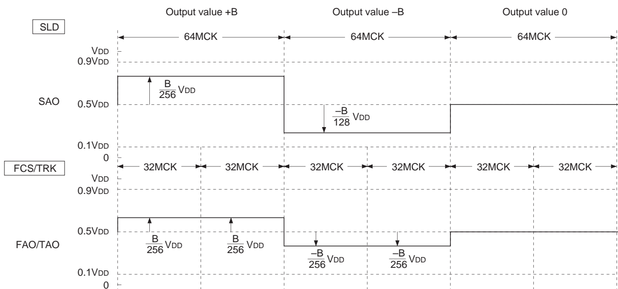
Timing Chart 5-22.
