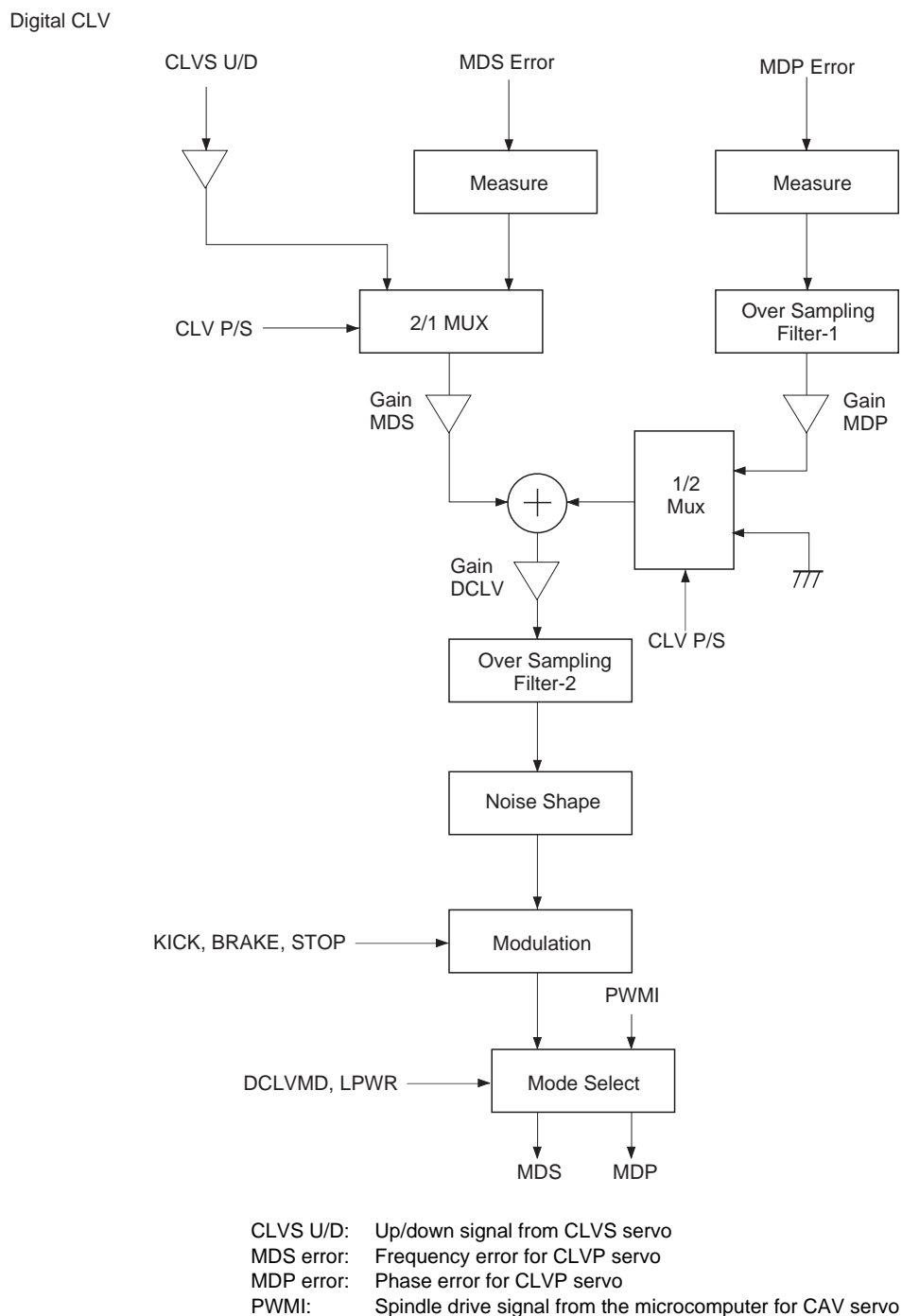
Fig. 4-14. Block Diagram
