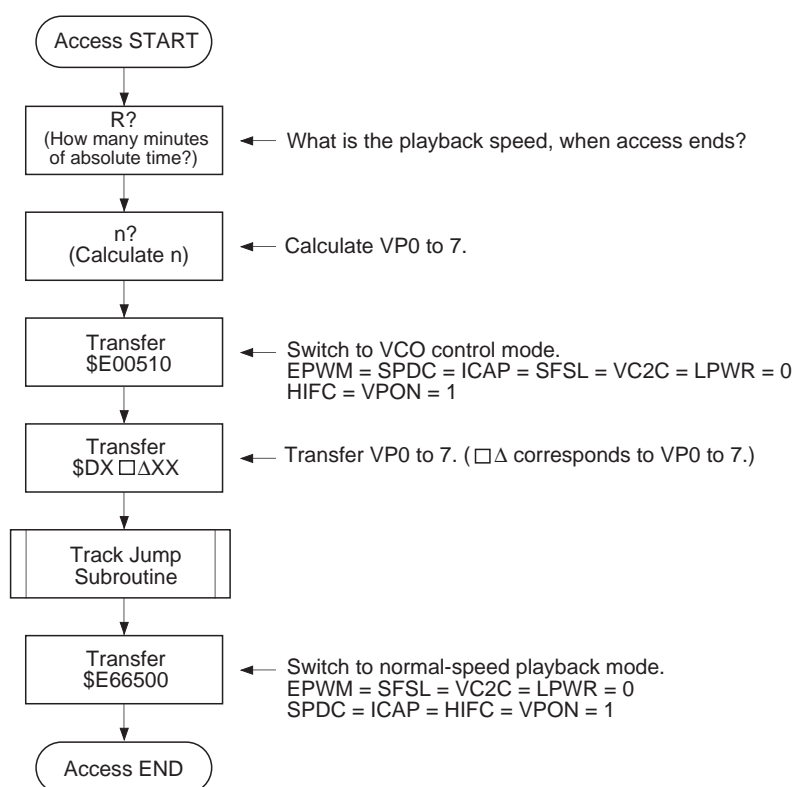
Fig. 3-3. Access Flow Chart Using VCO Control
