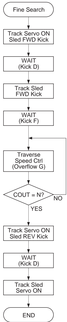
Fig. 4-12-(a). Fine Search Flow Chart
