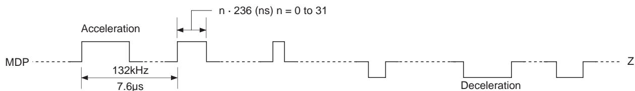
Timing Chart 1-8
