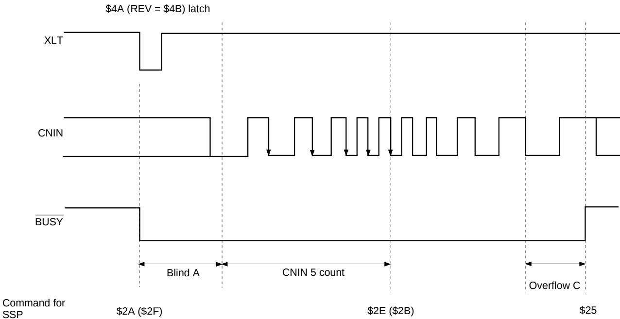
Fig. 4-5-(b). 10-Track Jump Timing Chart
