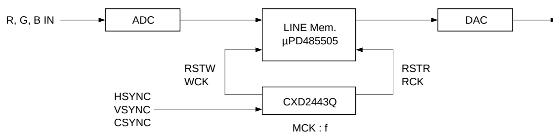
Double-speed display system block
