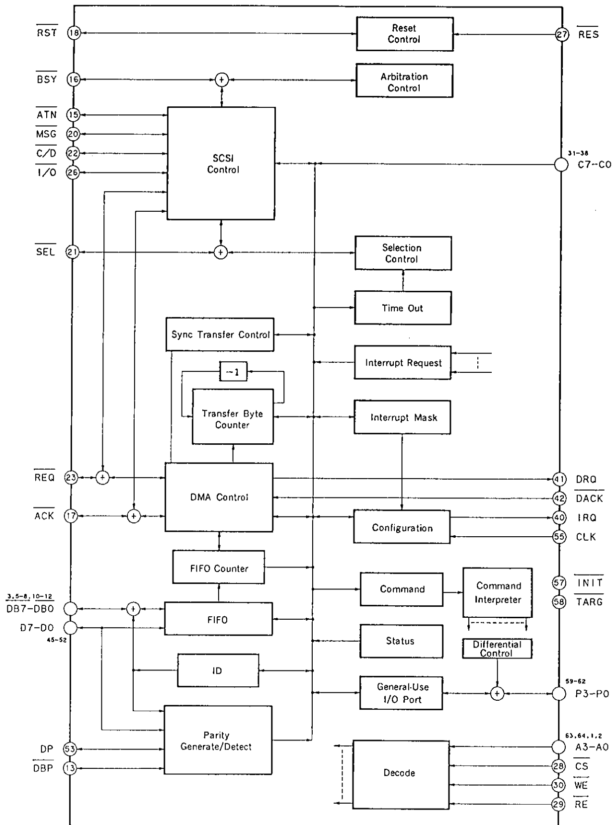
Block Diagram (CXD1185CR)
