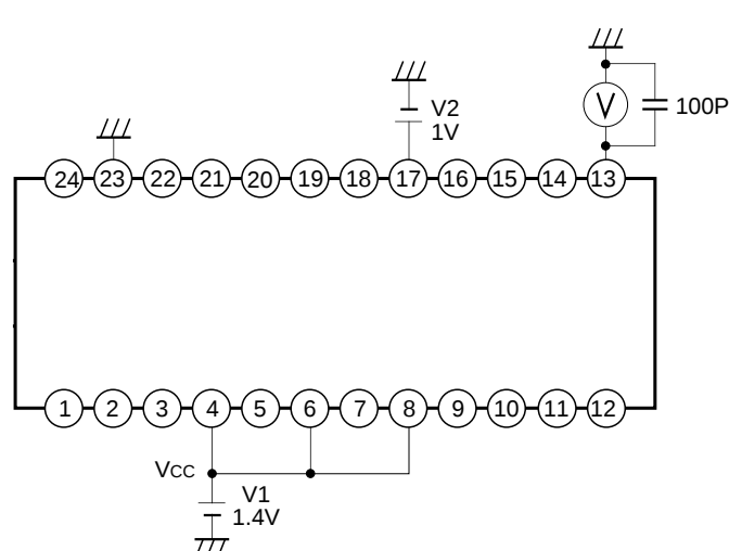
Measurement circuit 10
