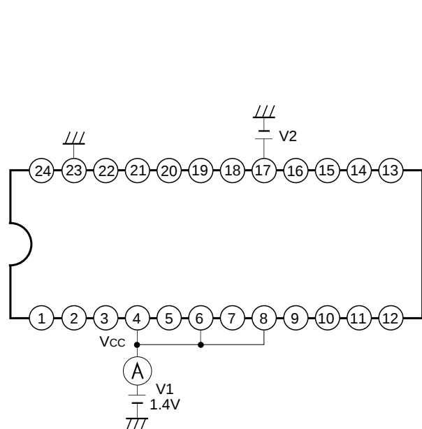
Measurement circuit 1
