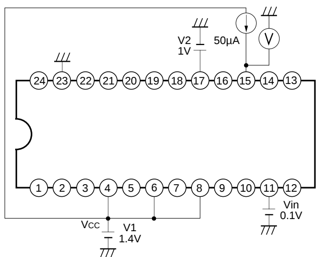
Measurement circuit 9
