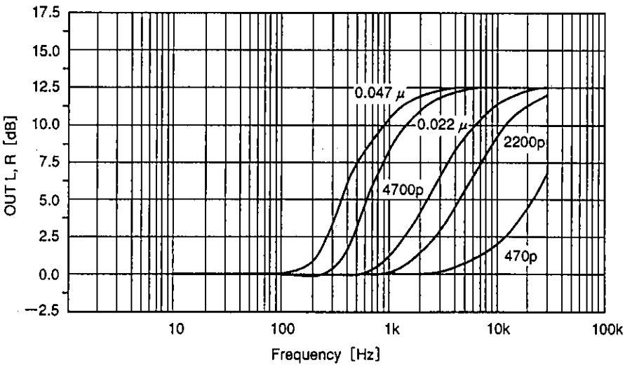
CH. vs. TREBLE-CONTROL (MAX)
