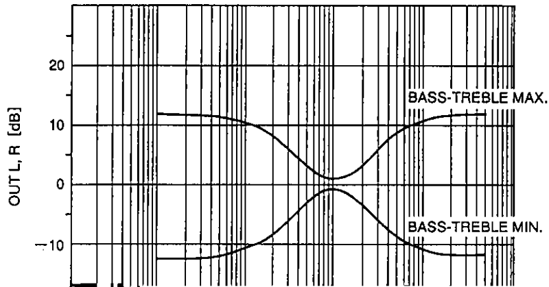
TONE characteristics
