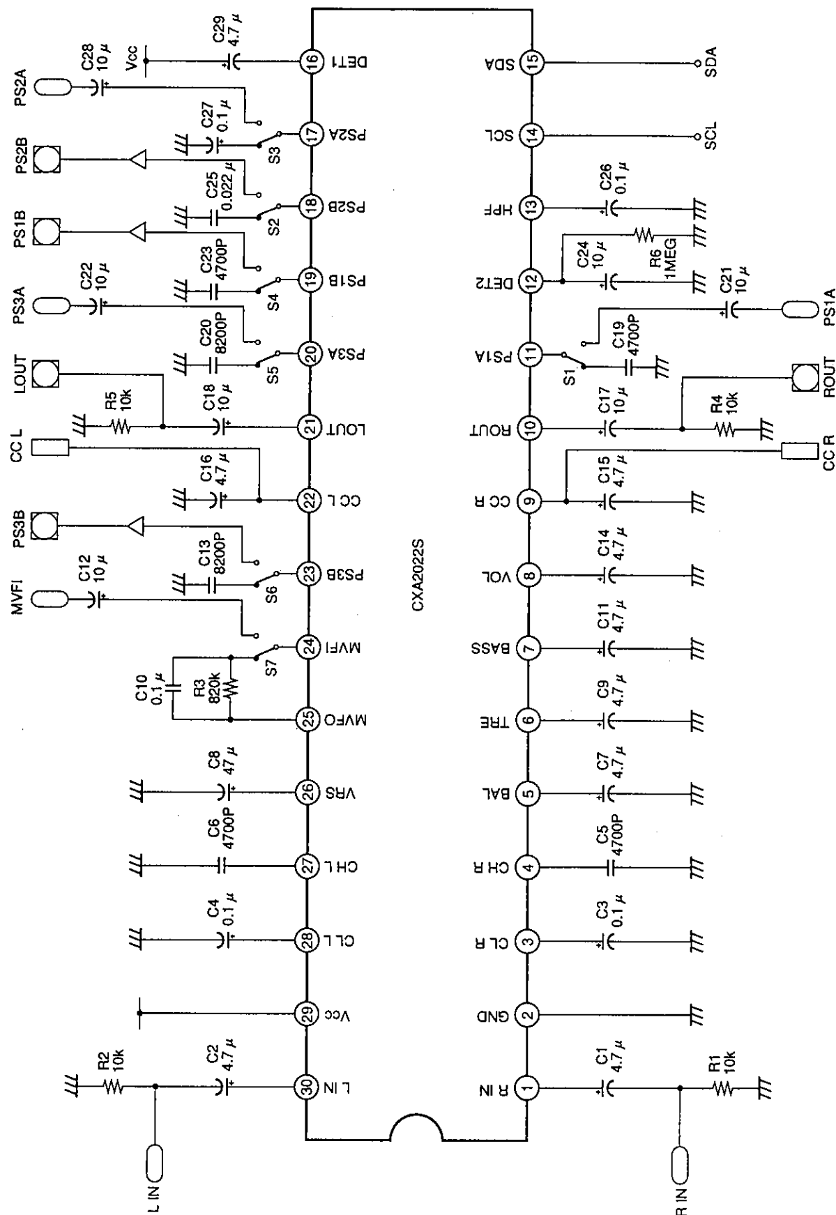
Electrical Characteristics Measurement Circuit
