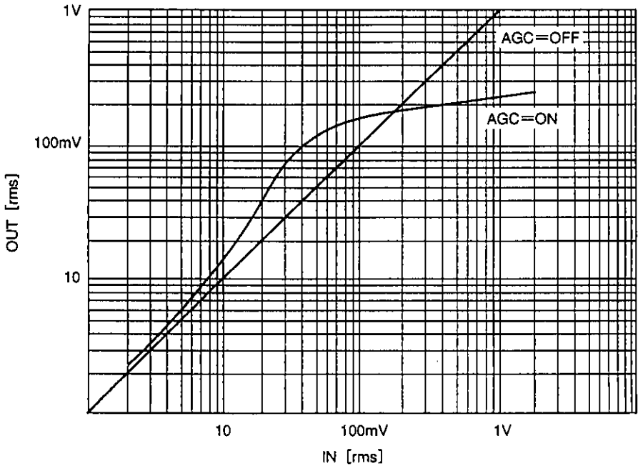
AGC characteristics
