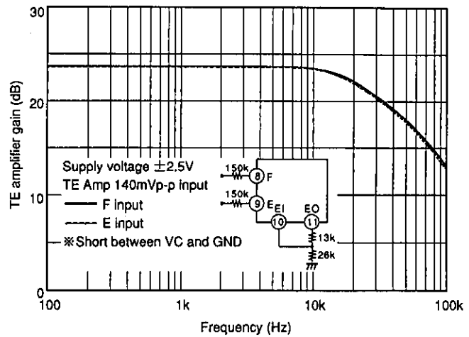
TE amplifier frequency characteristics (Frequency response comparison for F input and E input)
