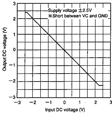
FE adjustment range characteristics
