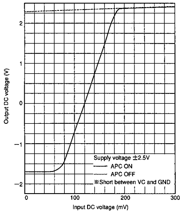
APC I/O voltage characteristics
